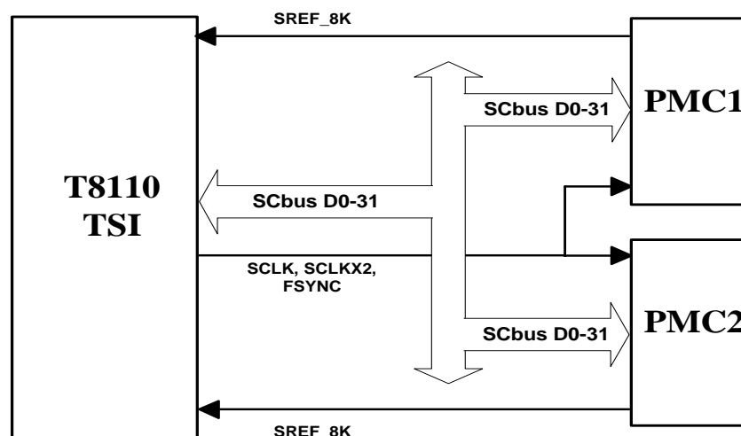
Figure 7: T8110 local TDM bus to shared SCbus Routing
