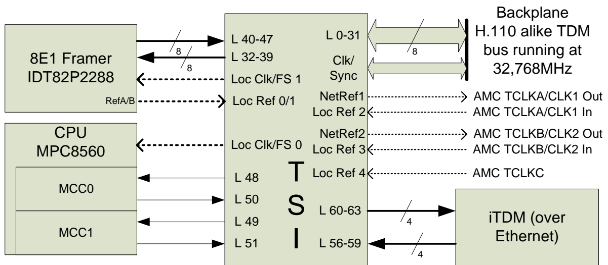
Figure 7: TSI TDM Interconnect
