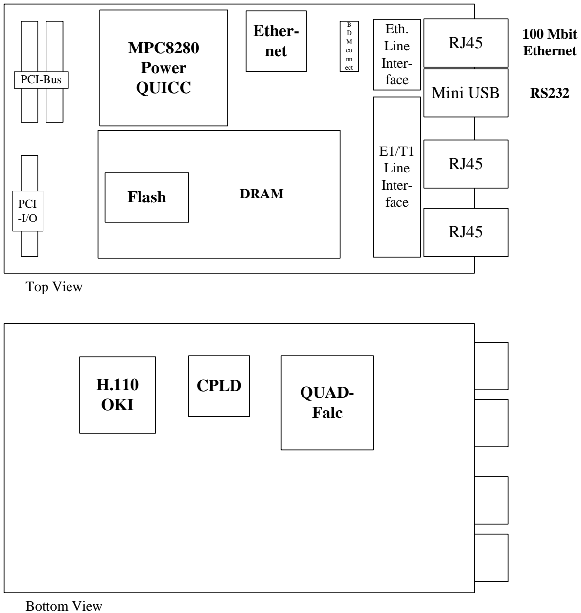
Figure 3: Location diagram of the NPMC-8280-4E1/T1/J1
