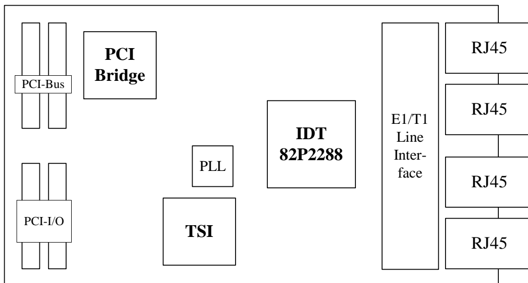
Figure 3: Location diagram of the NPMC-8E1/T1/J1
