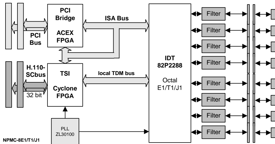
Figure 2: NPMC-8E1/T1/J1 Block Diagram
