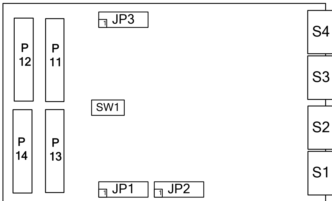
Figure 6: Connectors of the NPMC-8E1/T1/J1
